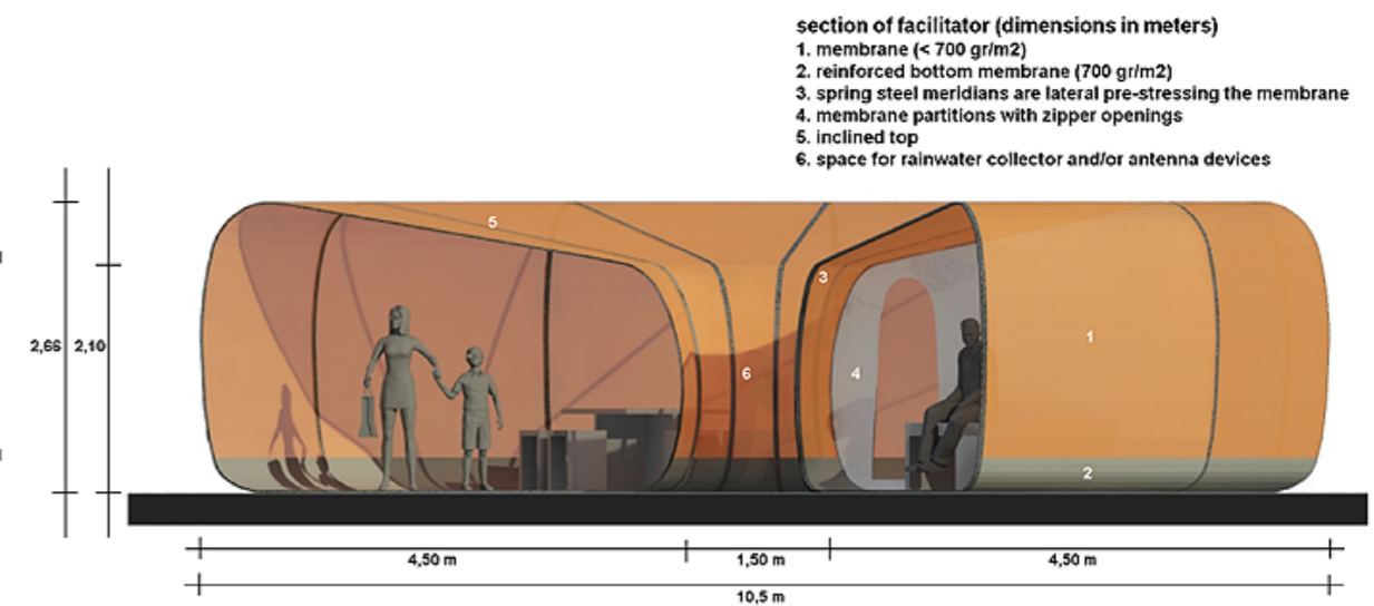
section of facilitator (dimensions in meters)
